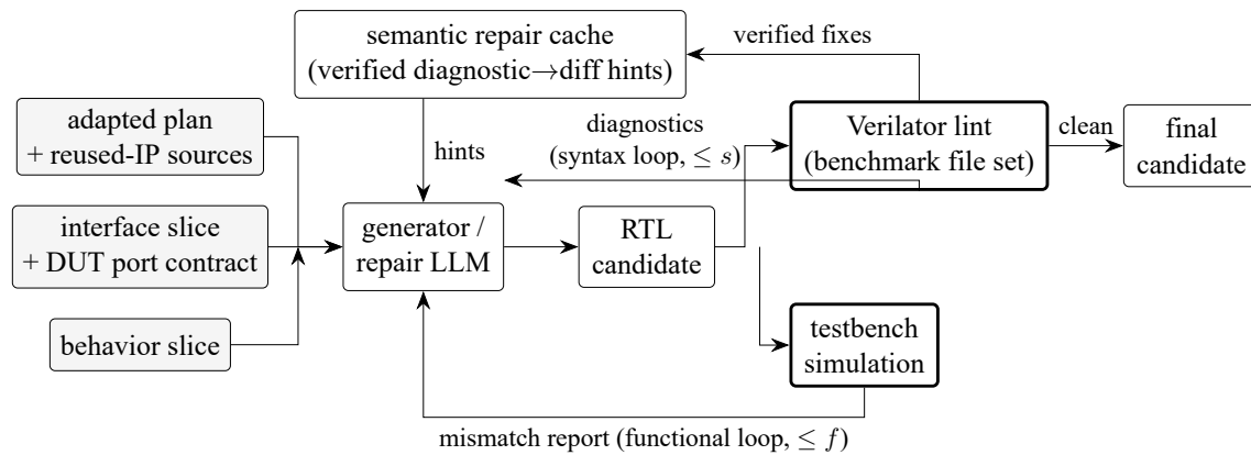
Figure 3.3: The generator’s verify-and-repair loop. A candidate first iterates in the syntax repair loop against the benchmark-faithful Verilator lint (budget s ), with the semantic repair cache injecting verified diagnostic→fix hints and absorbing new ones; compiling candidates then enter the functional repair loop against the testbench (budget f ), which keeps the best compiling candidate by mismatch count. Interface and behavior slices of the specification target each loop’s prompt.
