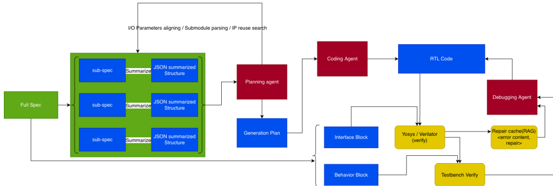
Figure 3.1: Dataflow of the two-stage pipeline. The specification is split into sub-specs and summarized into structured form, which the planning agent merges into a generation plan (left). The coding agent consumes the plan and produces RTL inside a Yosys/Verilator syntax repair loop backed by the semantic repair cache, followed by testbench-driven functional repair through the debugging agent (right). Interface and behavior slices of the specification feed the verification and repair loops.
