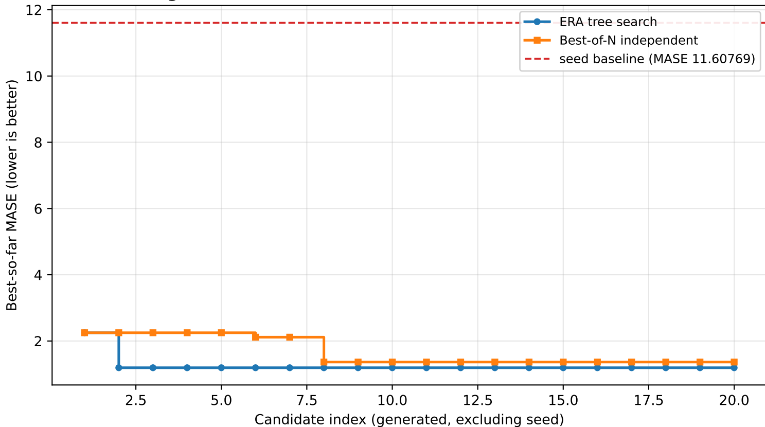
C4: ERA vs Best-of-N on GIFT-Eval m4_hourly/H/short best generated-candidate MASE so far (N=20, lower is better)
