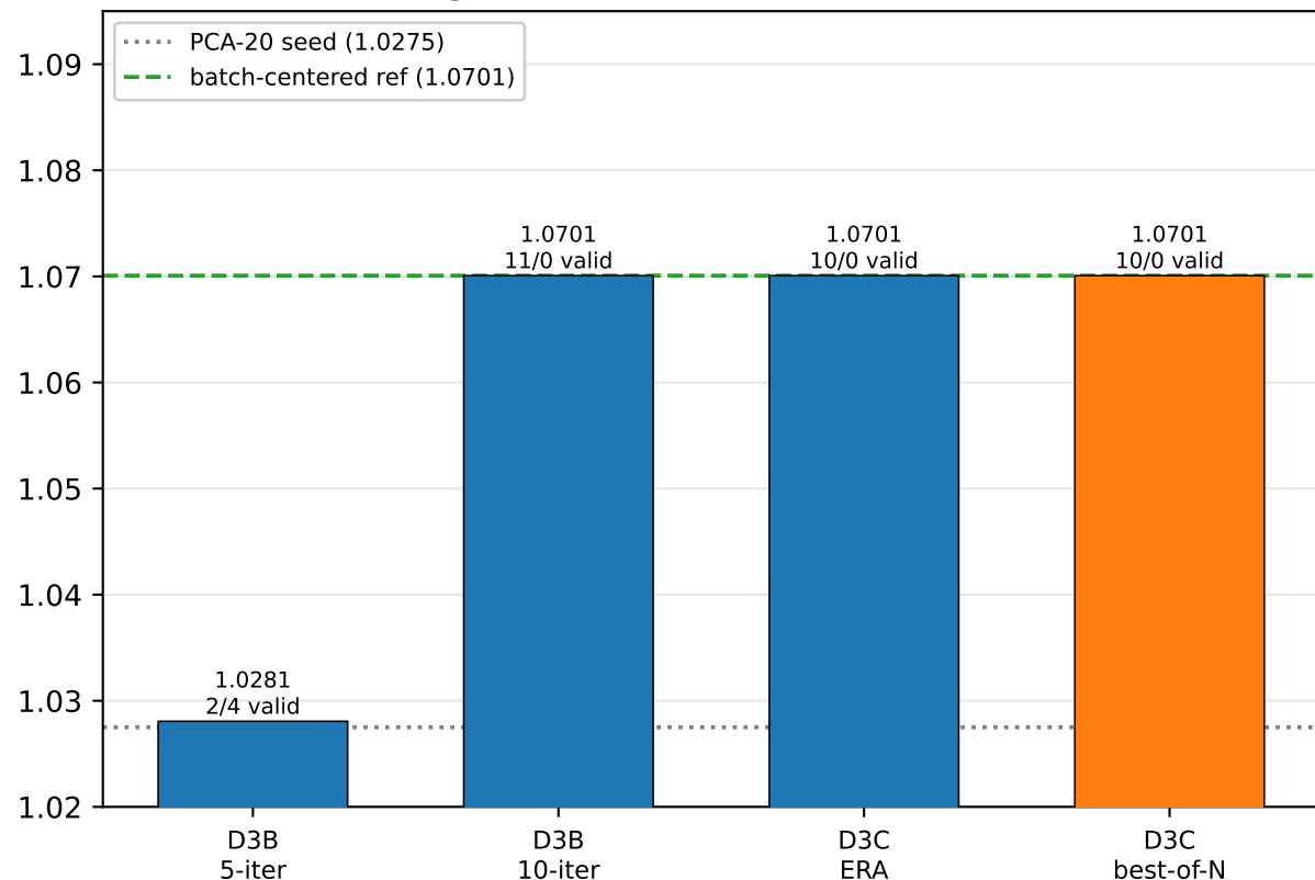
B. PBMC3k real bridge (D3A baselines + D3B ERA + D3C ERA-vs-BoN)
