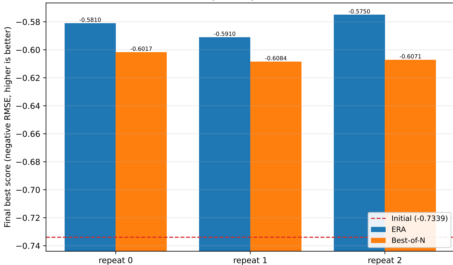
Final Best Score per Repeat: ERA vs. Best-of-N
