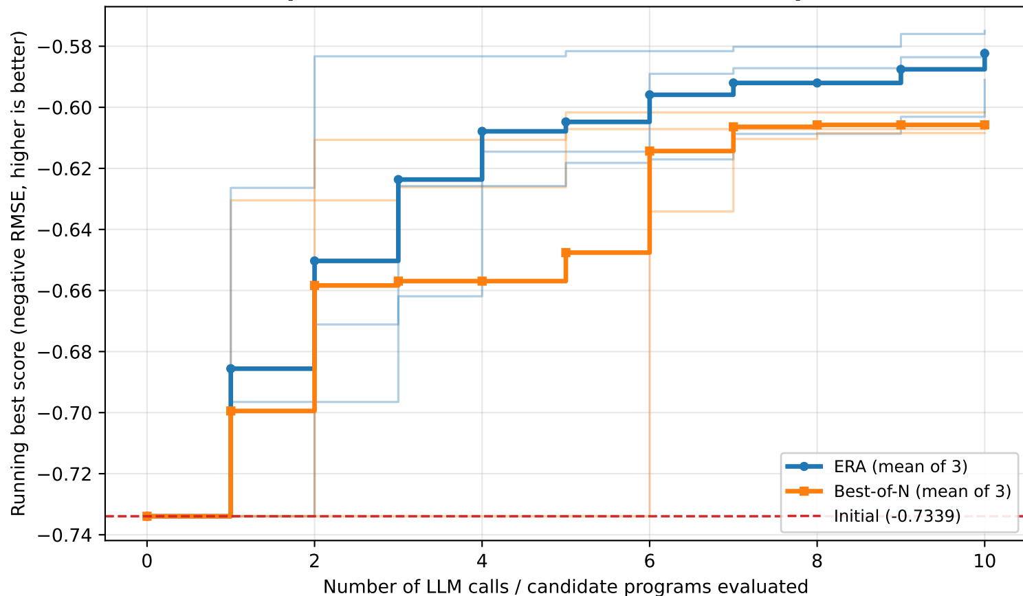
Repeated ERA vs. Best-of-N (N=10, 3 repeats)
