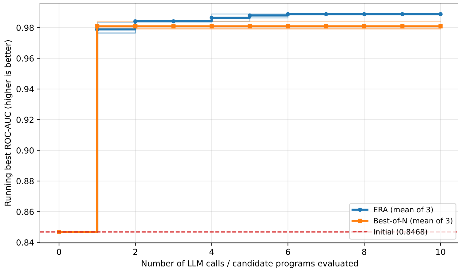
Breast Cancer: Repeated ERA vs Best-of-N (N=10, 3 repeats)
