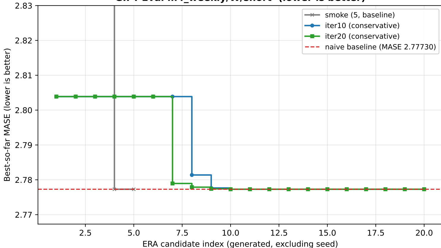
C3: best generated-candidate MASE so far (excl. naive seed) GIFT-Eval m4_weekly/W/short (lower is better)
