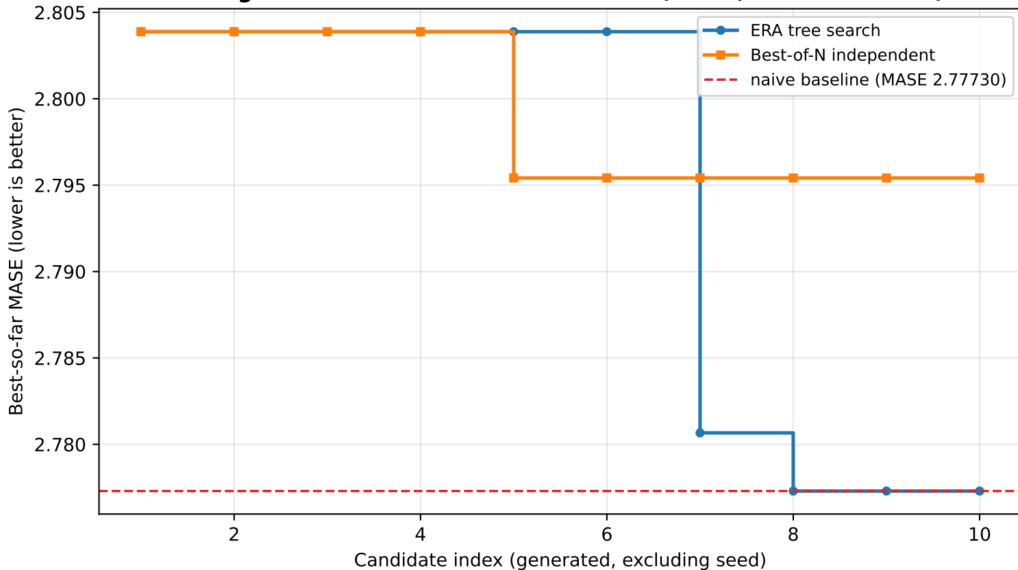
C4: ERA vs Best-of-N on GIFT-Eval m4_weekly/W/short best generated-candidate MASE so far (N=10, lower is better)
