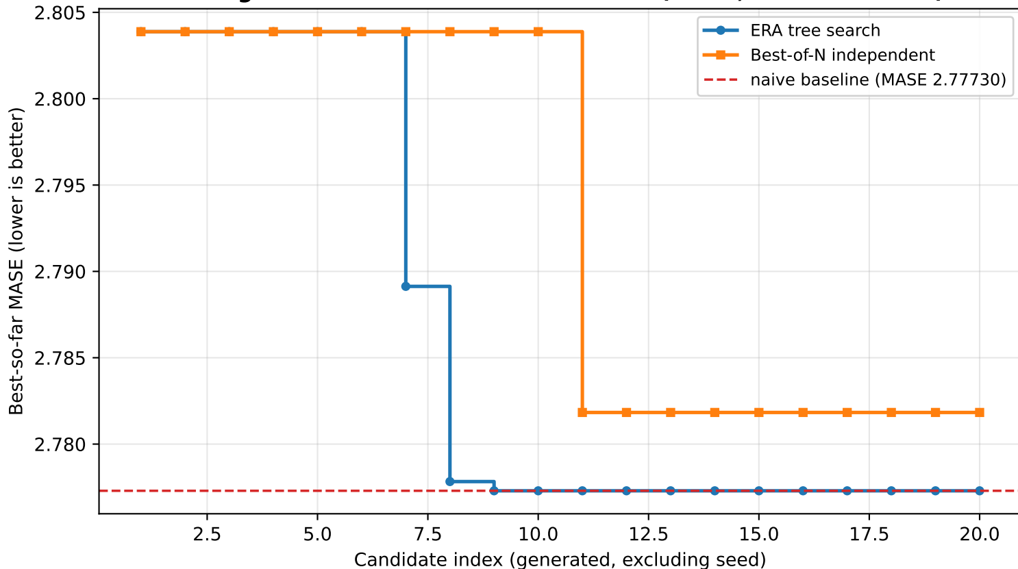
C4: ERA vs Best-of-N on GIFT-Eval m4_weekly/W/short best generated-candidate MASE so far (N=20, lower is better)
