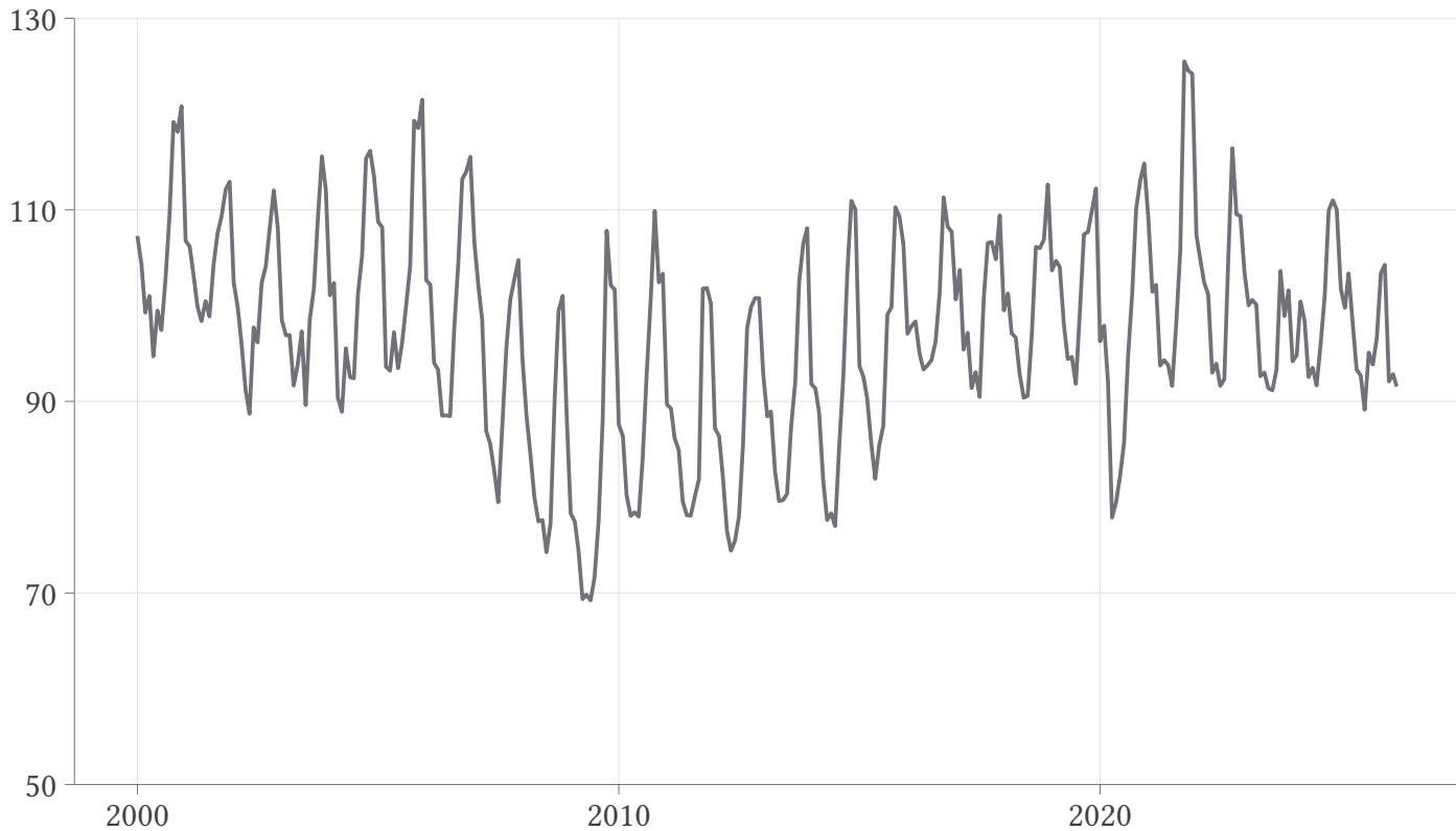
U.S. Candy Production
