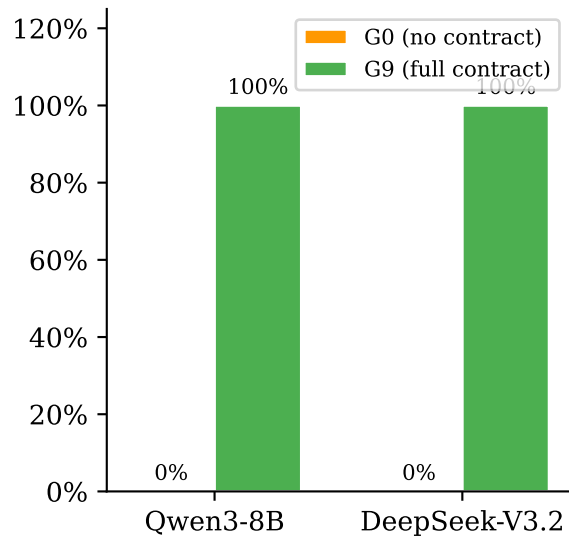
(a) Pass Rate
