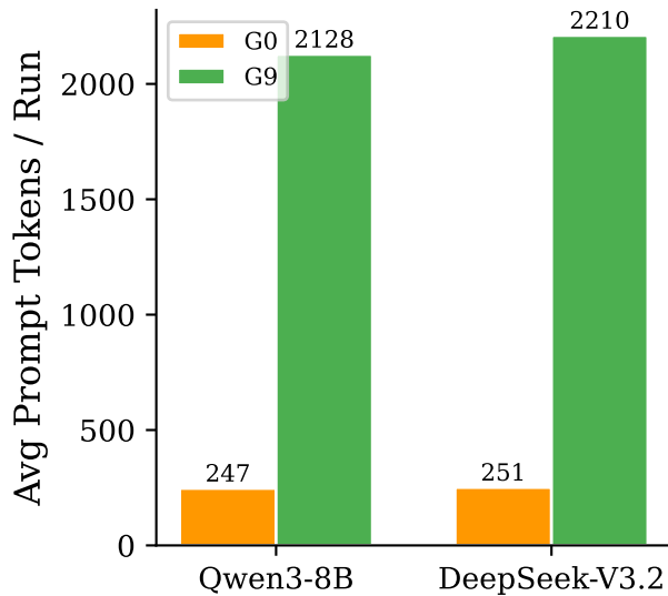
(b) Prompt Cost
