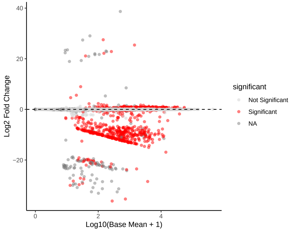
MA Plot: KO_M vs HT_F with Log10 Base Mean
