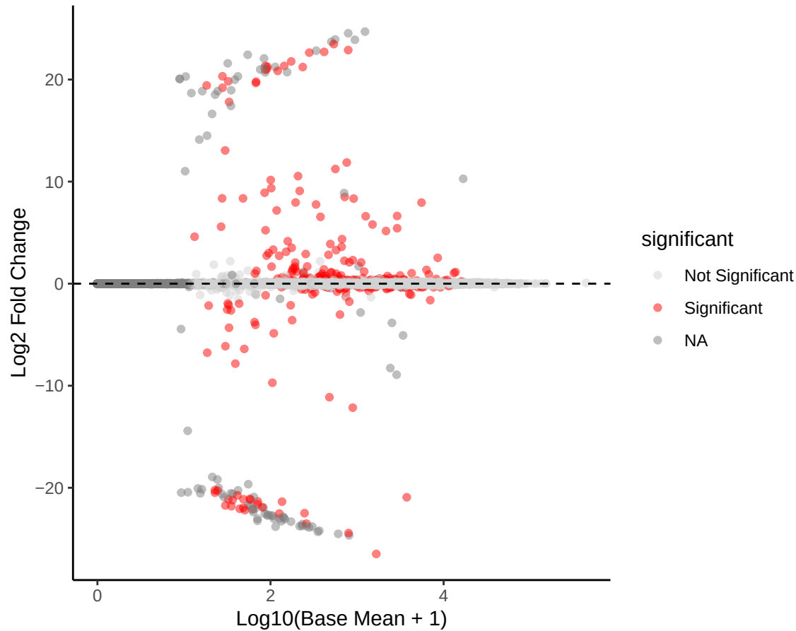
MA Plot: KO_M vs WT_M with Log10 Base Mean
