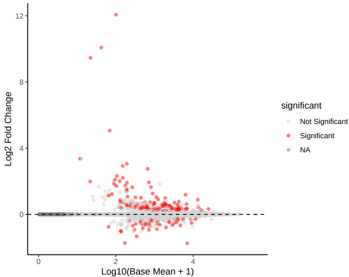
MA Plot: Mut vs WT with Log10 Base Mean
