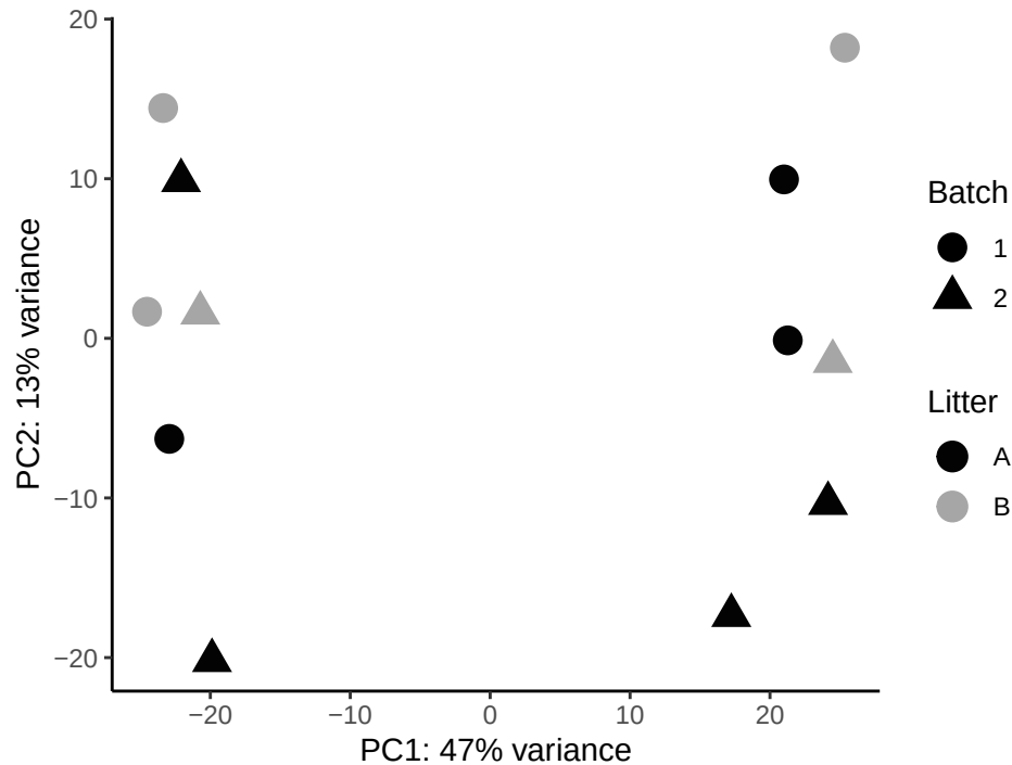
PCA Plot of Mice Litter and RNA Extraction Batch
