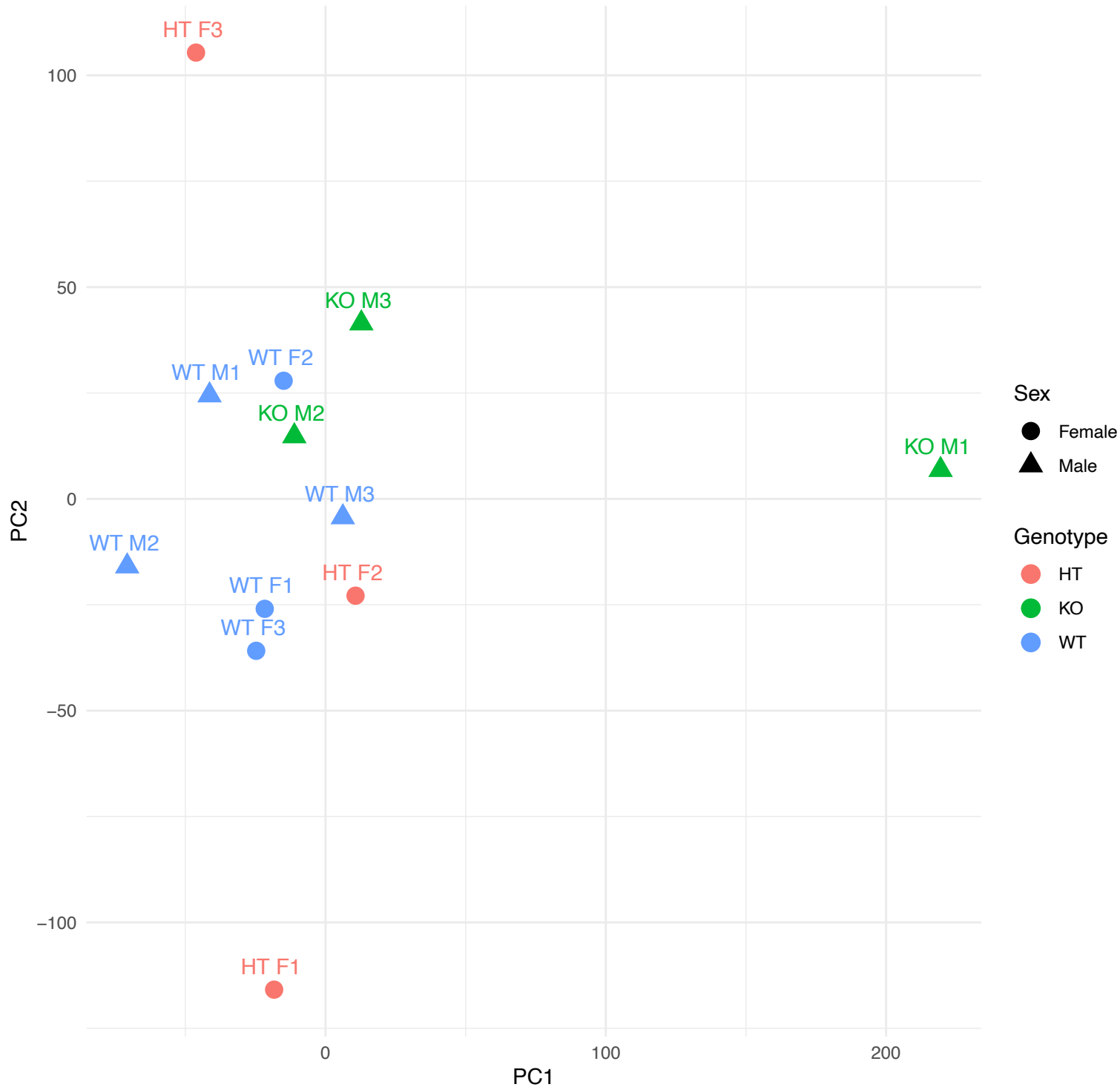
PCA of RNA-seq Samples
