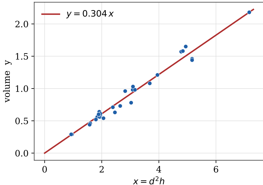
Black cherry tree data with no-intercept least-squares line
