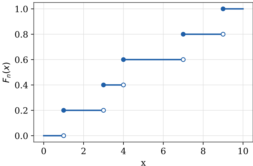
Empirical distribution function of \{1, 3, 4, 7, 9\}
