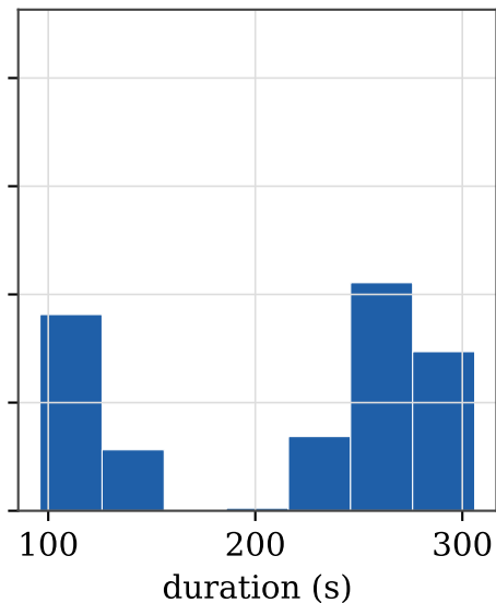
Histograms of the Old Faithful durations for three bin widths
