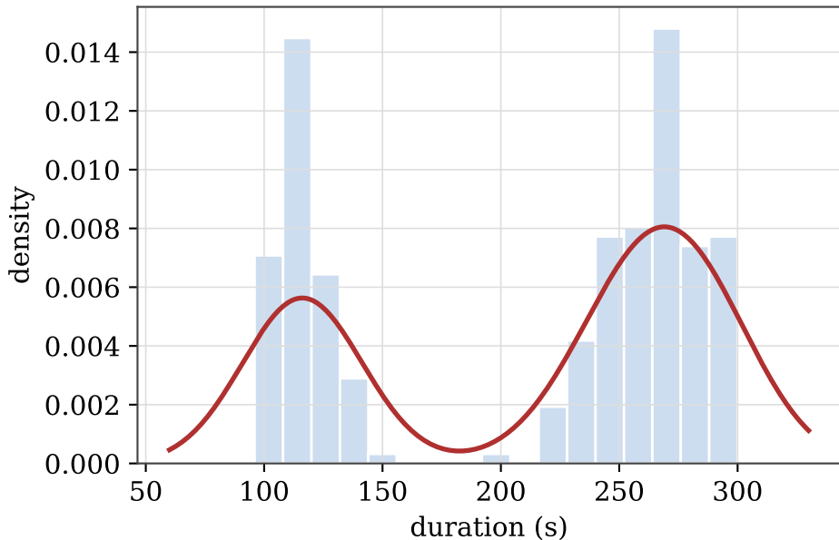
Kernel density estimate of the Old Faithful data
