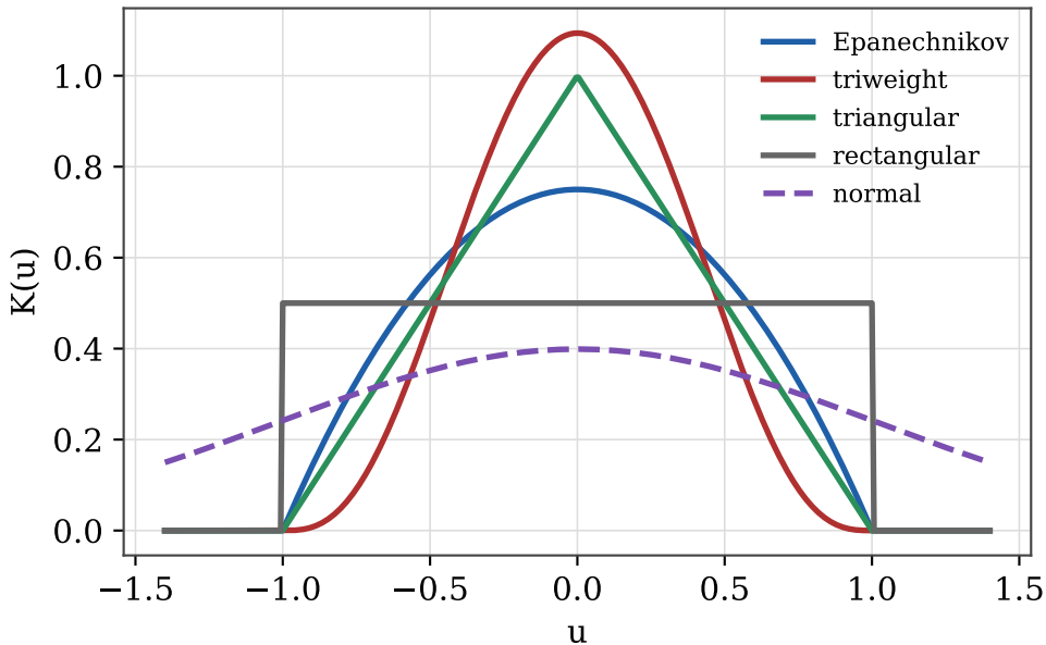
Several well-known kernels
