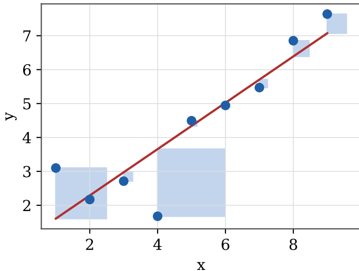
Deviations from the line ( SS_{res} )
