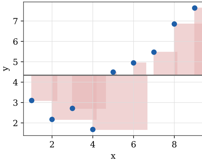
Deviations from the mean \bar{y} ( SS_{tot} )
