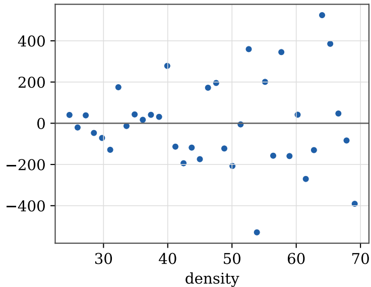
Quadratic model: residuals fan out
