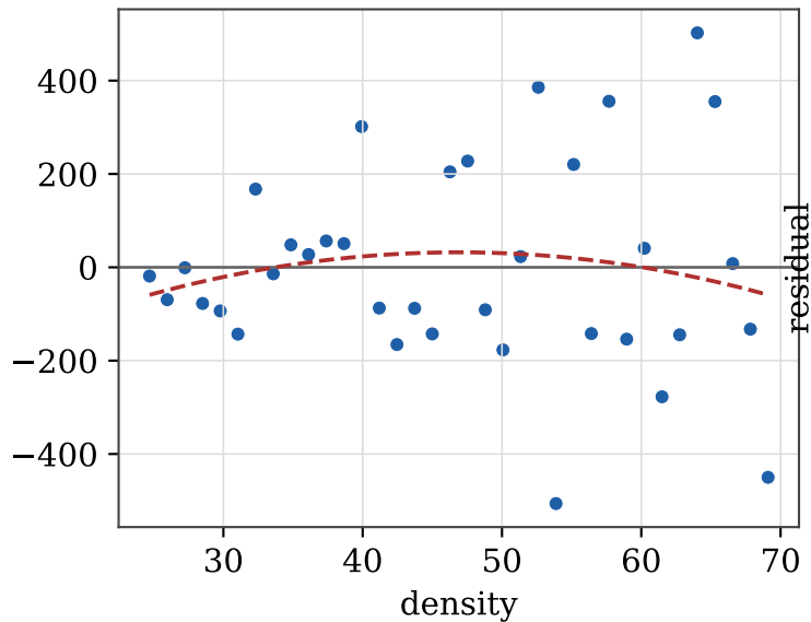
Linear model: residuals bend (parabolic)
