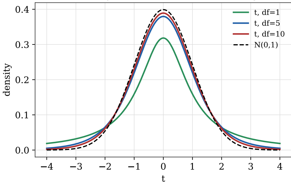
The t density approaches N(0,1) as df grows
