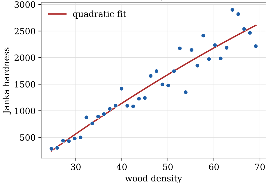
Janka hardness versus density (illustrative timber data)
