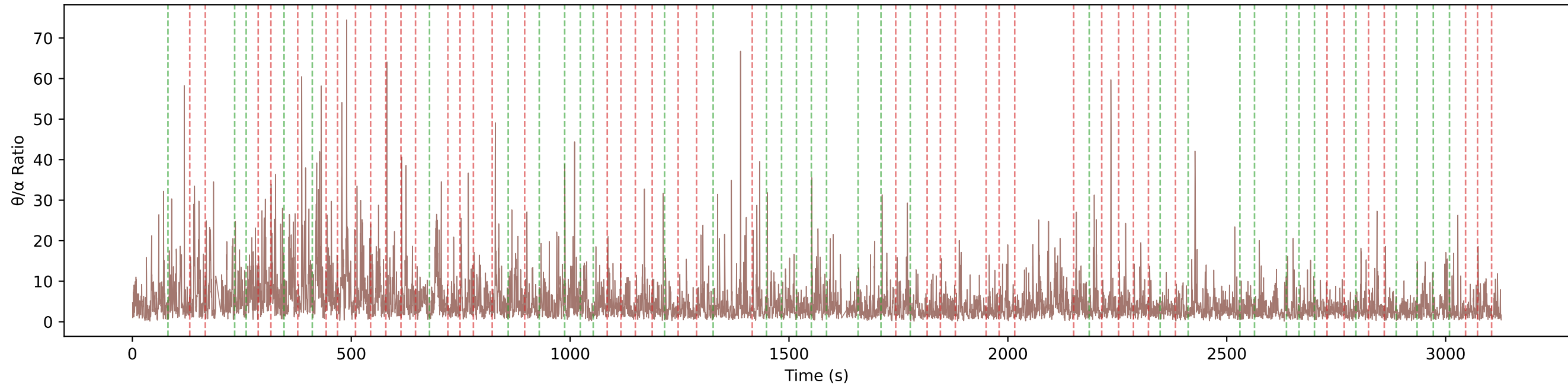
Pre-Shot \theta/\alpha Ratio by Outcome
