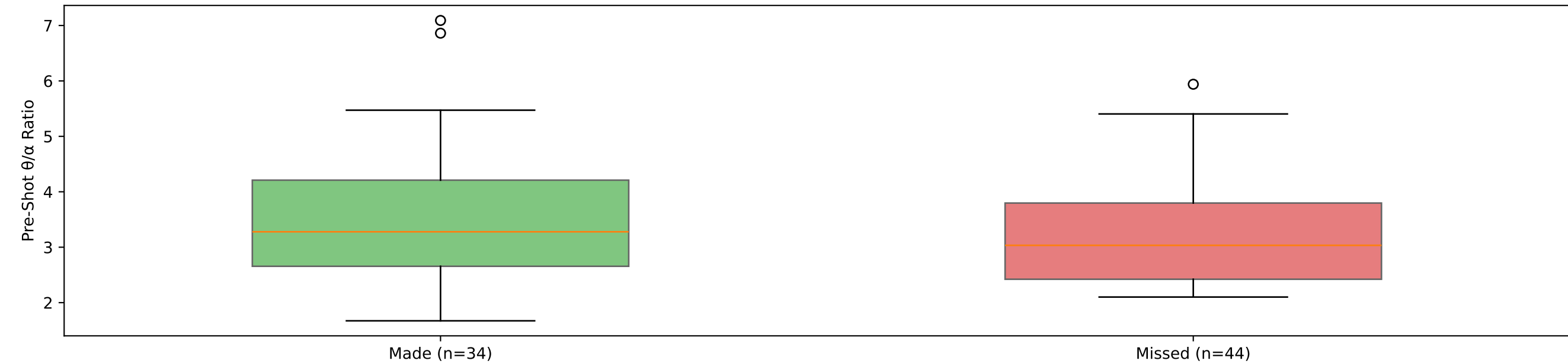
Pre-Shot \theta/\alpha Ratio by Outcome
