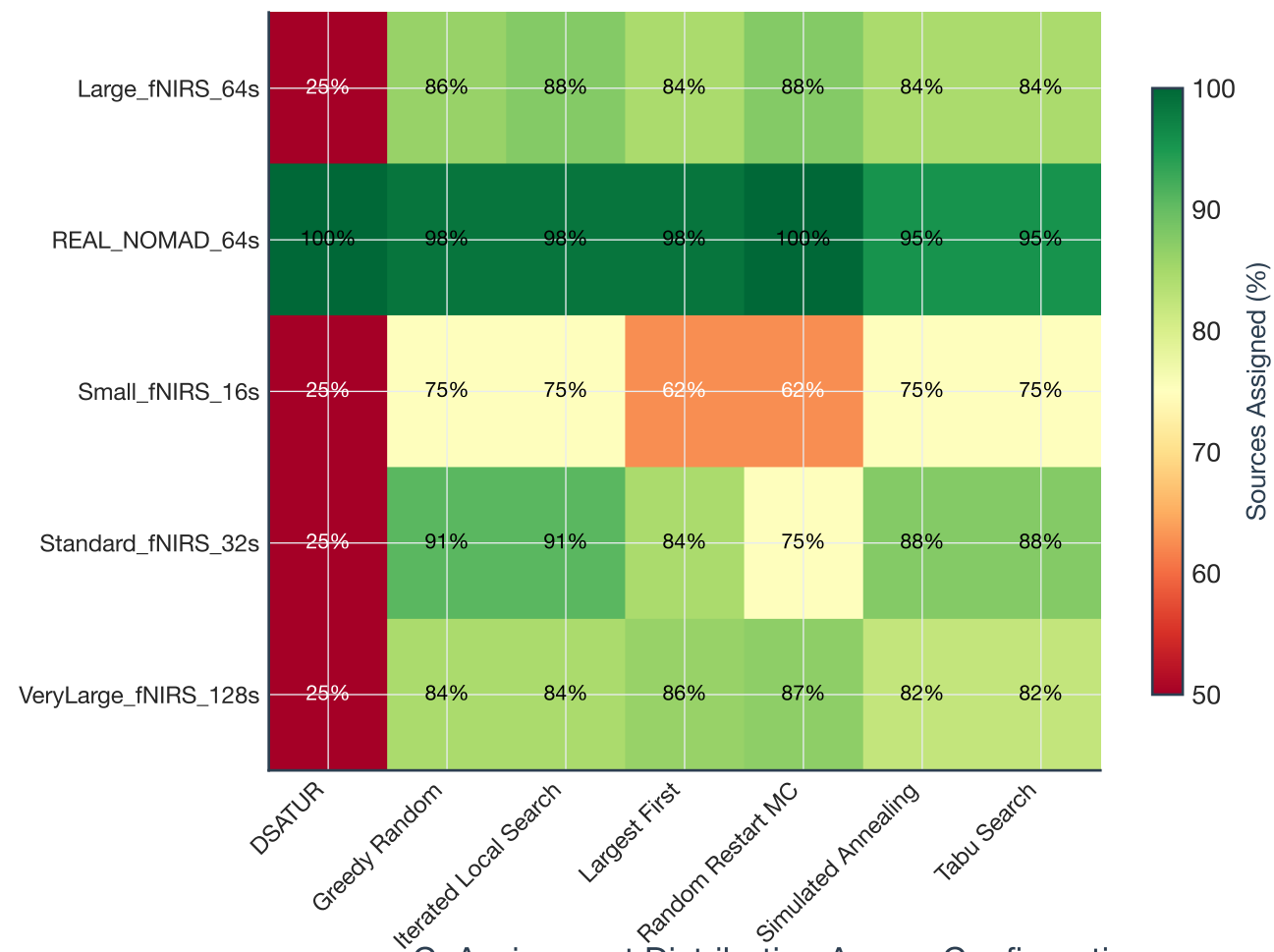
C. Assignment Distribution Across Configurations
