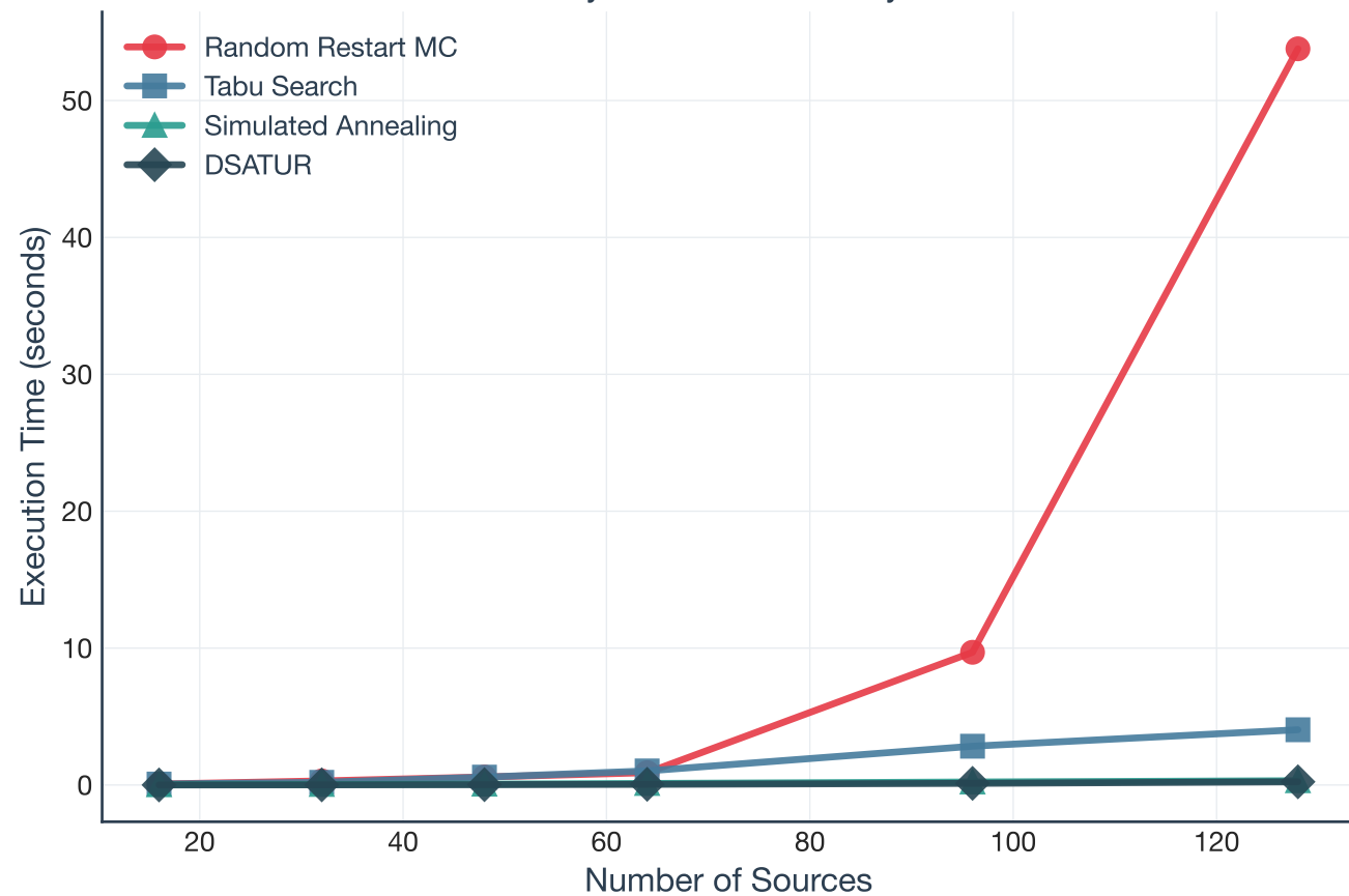
A. Scalability: Time vs fNIRS System Size
