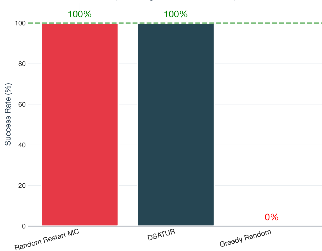
Success Rate on REAL_NOMAD_64s (% finding COMPLETE solution)
