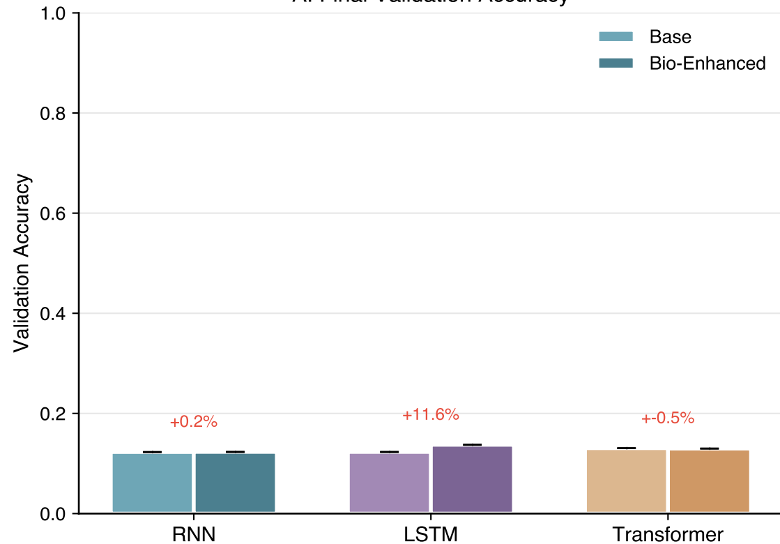
A. Final Validation Accuracy
