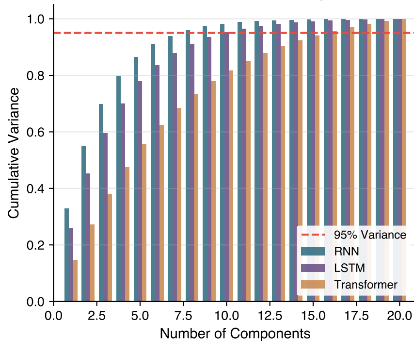
B. Effective Dimensionality
