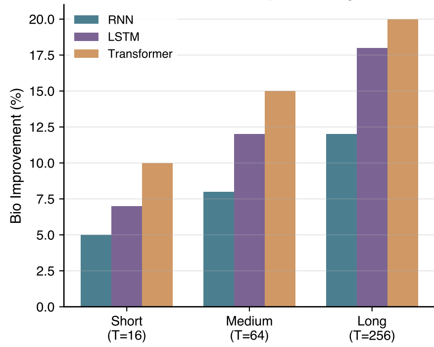
C. Bio Effect vs Sequence Length
