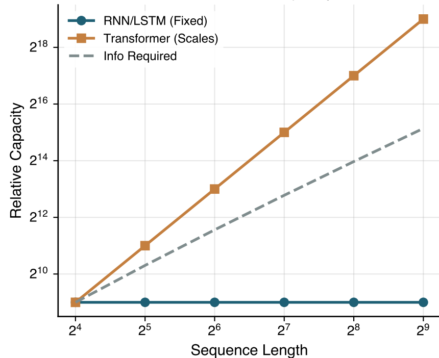
A. Information Capacity
