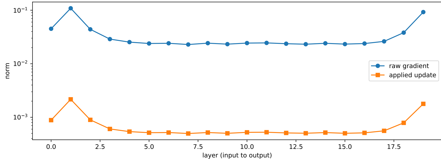
depth_L20_theopoula, iteration 50000
