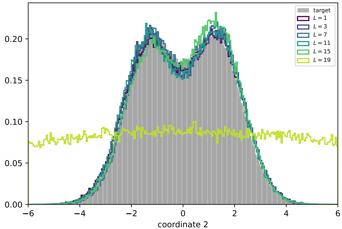
depth sweep, adam
