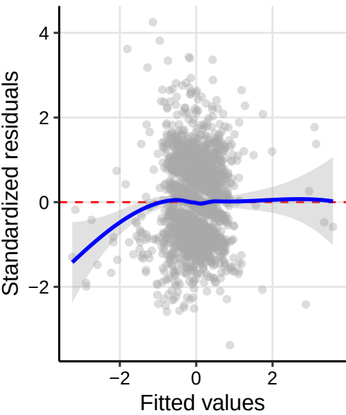
Residuals vs Fitted Values
