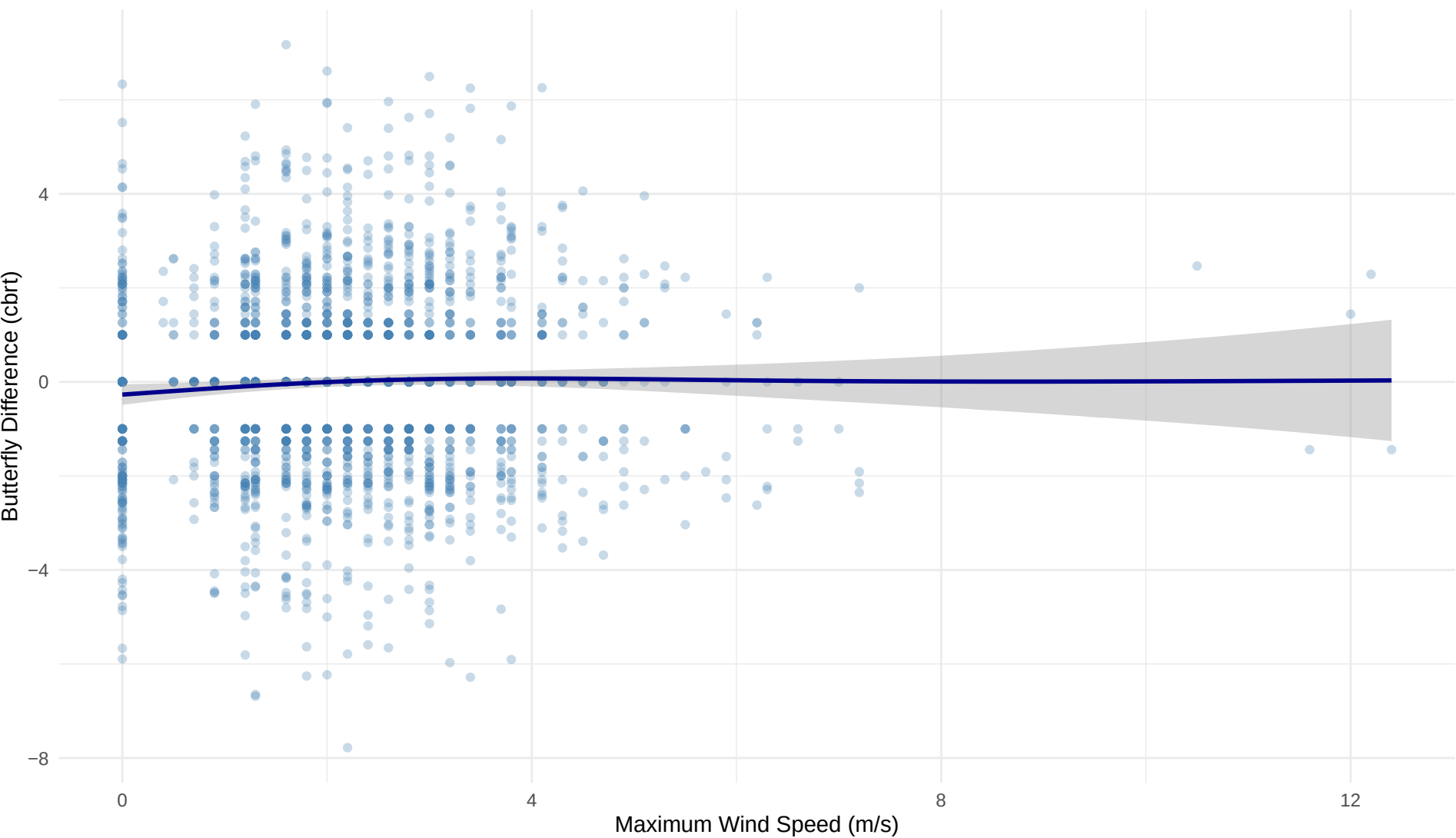
Maximum Wind Speed vs Butterfly Change
