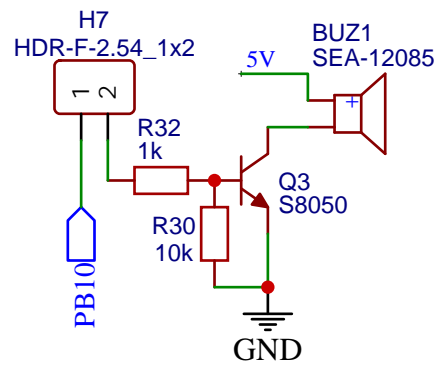
Buzzer
