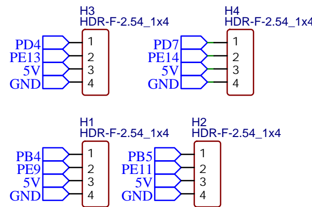
Reserved Interface
