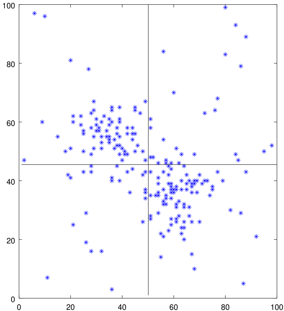
Simple mean, ONE CLUSTER
