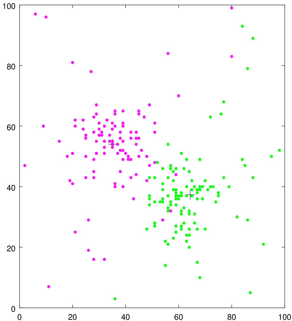
Finished K-Means
