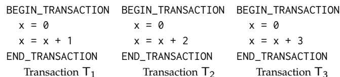
Figure 7.12: Three transactions.
