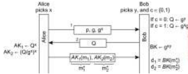
Figure 9.6: A simple 1-out-of-2 oblivious transfer.
