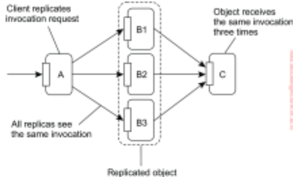
Figure 7.28: The problem of replicated object invocations.
