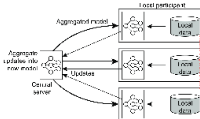
Figure 3.26: The principle of federated learning.
