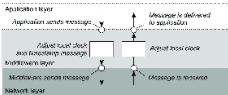
Figure 5.8: The positioning of Lamport's logical clocks in distributed systems.
