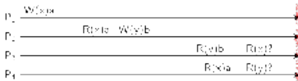
Figure 7.10: A slight modification of Figure 7.9(a). What should R_3(x) or R_4(y) return?
