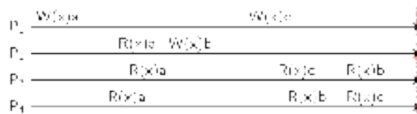
Figure 7.8: This sequence is allowed with a causally consistent store, but not with a sequentially consistent store.
