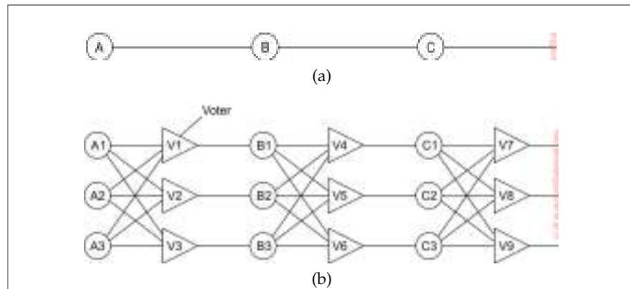
Figure 8.3: Triple modular redundancy.
