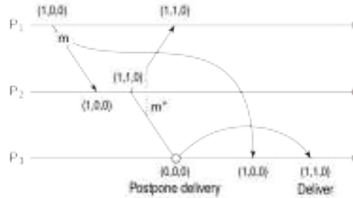
Figure 5.13: Enforcing causal communication.
