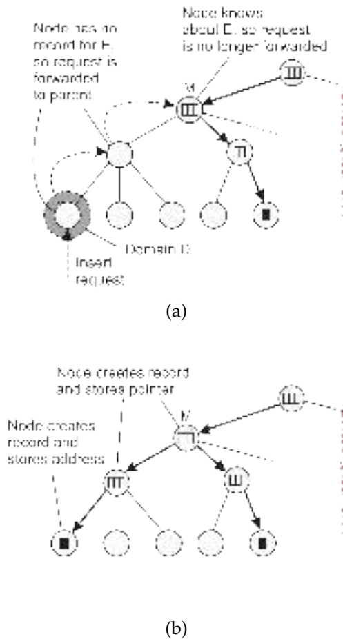
Figure 6.8: (a) An insert request is forwarded to the first node that knows about entity E. (b) A chain of forwarding pointers to the leaf node is created.
