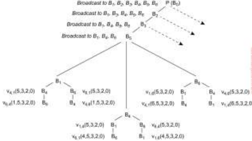
Figure 8.17: Rounds of broadcasting v_0 to the backups, by P and the backups B_1, \dots, B_6 .
