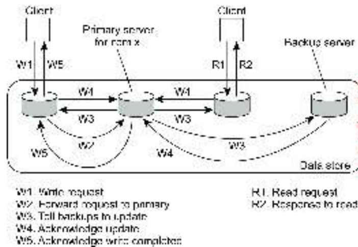
Figure 7.30: The principle of a primary-backup protocol.
