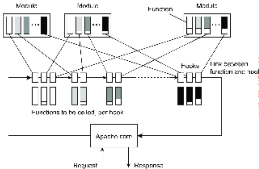
Figure 3.22: The general organization of the Apache Web server.
