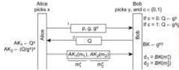
Figure 9.6: A simple 1-out-of-2 oblivious transfer.
