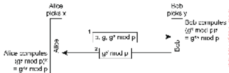
Figure 9.5: The principle of Diffie-Hellman key exchange.
