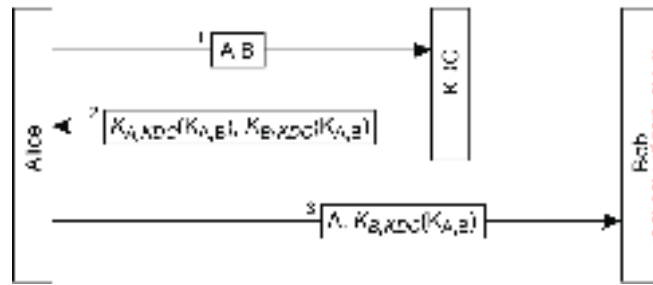
Figure 9.12: Using a ticket and letting Alice set up a connection to Bob.
