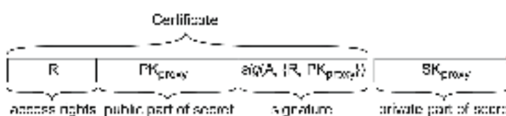
Figure 9.24: The general structure of a proxy as used for delegation.
