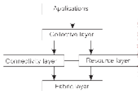
Figure 1.10: A layered architecture for grid computing systems.
