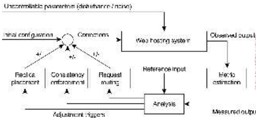
Figure 7.36: The general organization of a CDN as a feedback-control system.
