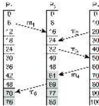
Figure 5.11: Concurrent message transmission using logical clocks.
