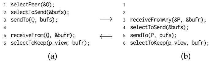
Figure 5.25: Communication between the (a) active and (b) passive thread in a peer-sampling service.
