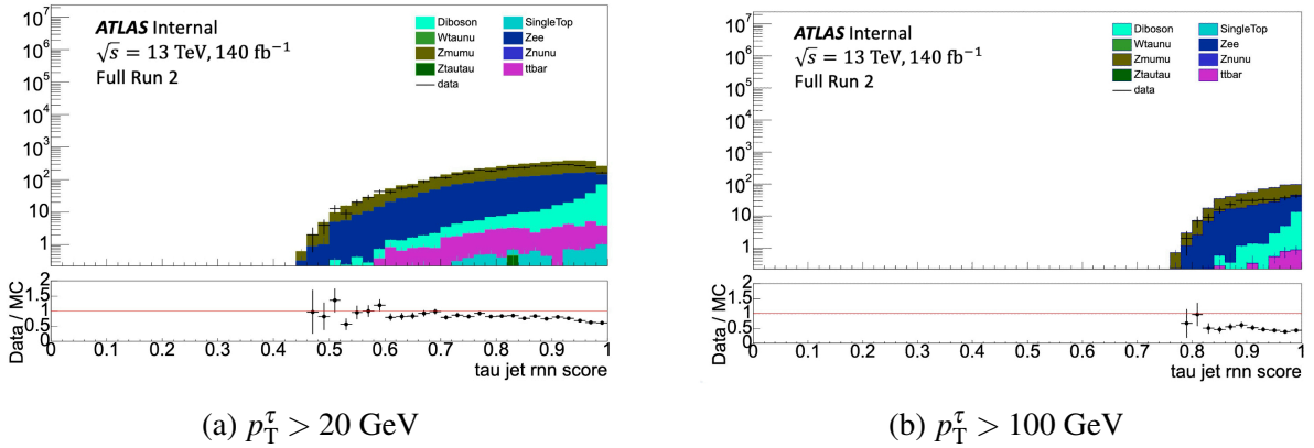
Fig. 8.7 The \tau -identification RNN score in Z+jets-enriched samples with (a) p_T^\tau > 20 GeV and (b) p_T^\tau > 100 GeV. Looser \tau identification and a relaxed transverse-mass requirement are used to compare the low- and high-score regions. These selections differ from the nominal ZVR.
