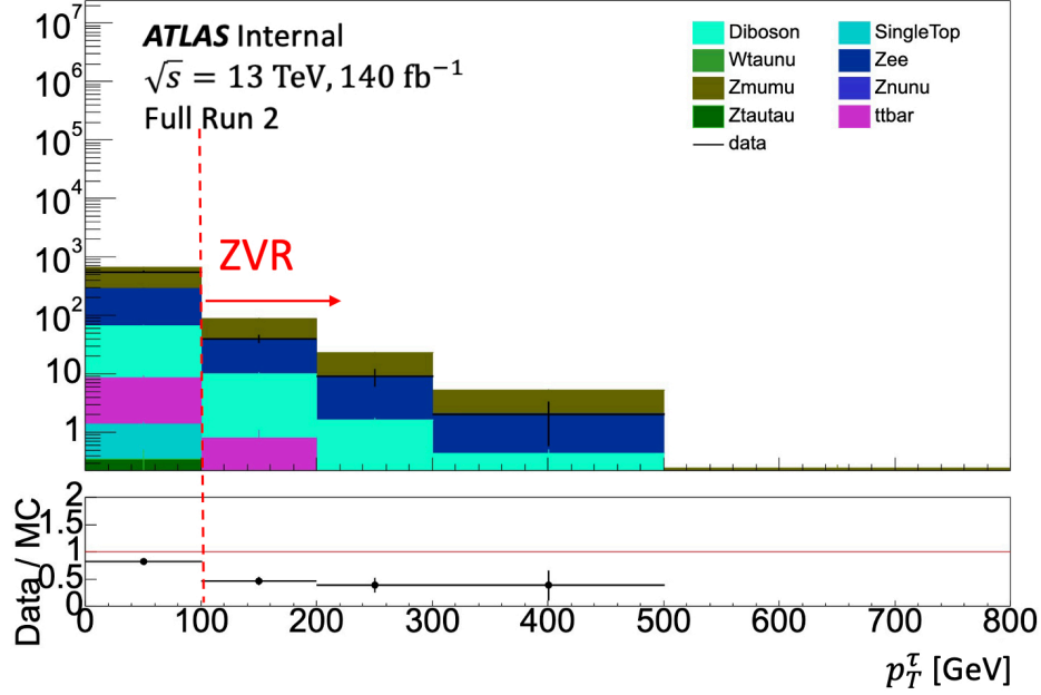
Fig. 8.6 Pre-fit N - 1 distribution of p_T^\tau in the ZVR. The red arrow indicates the 100 GeV threshold. The lower panel compares data with the total simulation. The high- p_T^\tau prediction exceeds the observed yield.
