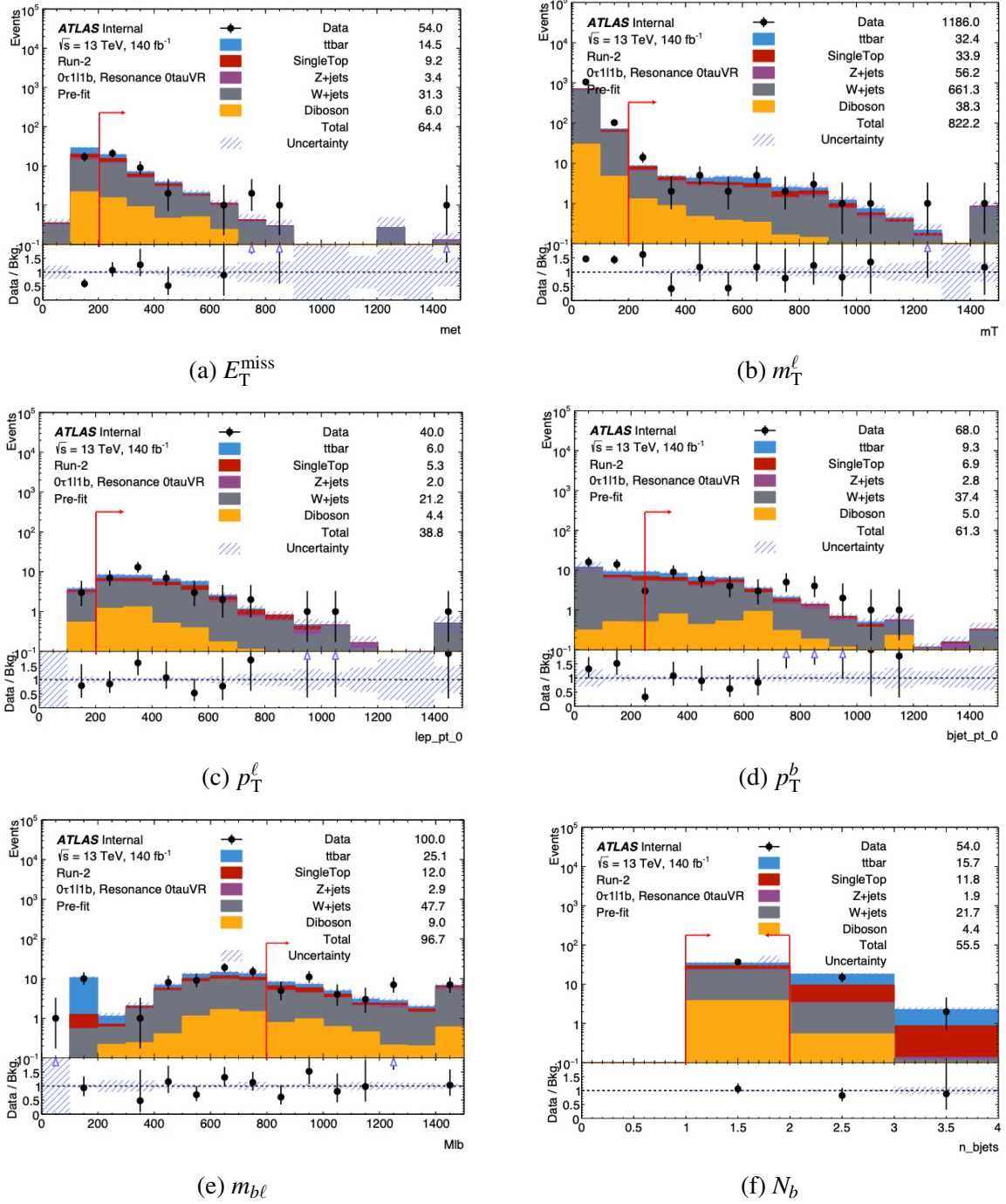
Fig. 8.8 Pre-fit N - 1 distributions in VRW-Res. The electron and muon channels are combined. The lower panels show data divided by the total simulated background. The hatched bands represent the statistical uncertainty in the prediction. The last bin includes the overflow. The original plot labels 0 \tau VR denote VRW.
