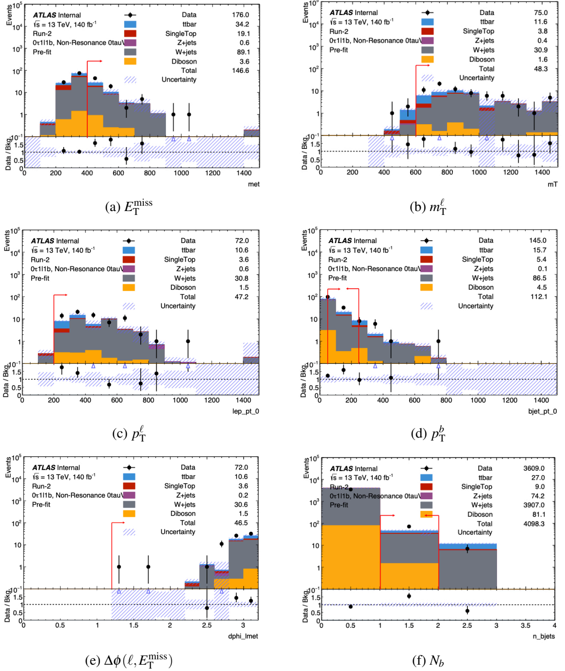
Fig. 8.9 Pre-fit N - 1 distributions in VRW-NonRes. The electron and muon channels are combined. The lower panels show data divided by the total simulated background. The hatched bands represent the statistical uncertainty in the prediction. The last bin includes the overflow. The original plot labels 0 \tau VR denote VRW.
