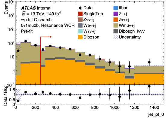
(b) p_T^j , \mu channel
