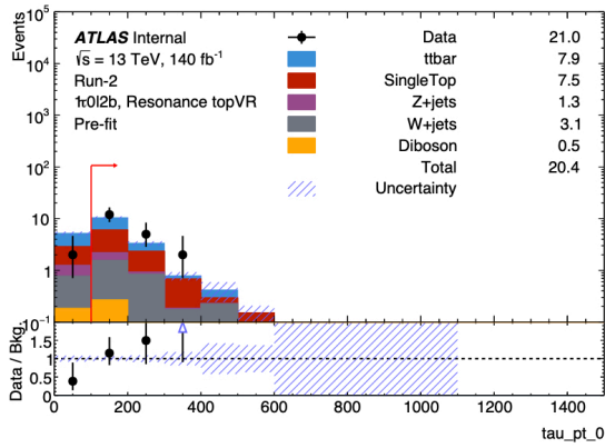
(c) p_T^{\tau}
