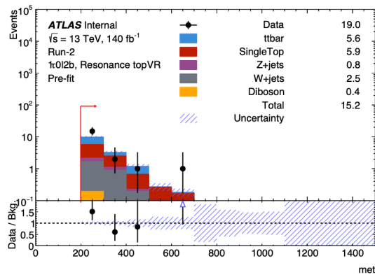
(a) E_T^{\text{miss}}
