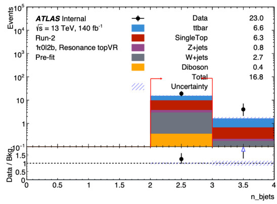
(f) N_b
