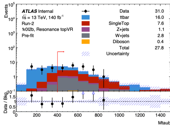
(e) m_{b\tau}
