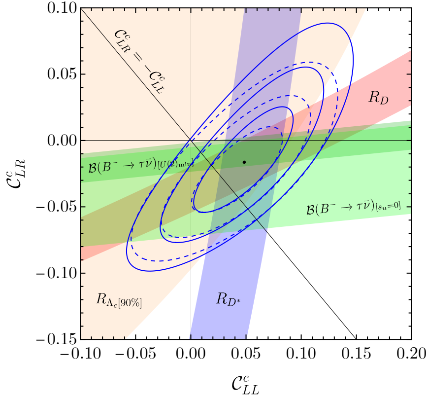
Fig. 3.1 The result in (C_{LL}^c, C_{LR}^c) plane obtained from the fit to low-energy b \rightarrow c\tau\nu observables. The blue solid ellipses correspond to the 1, 2 and 3 \sigma contours. The blue dotted lines are obtained including also the constraint from \mathcal{B}(B_u^- \rightarrow \tau\bar{\nu}) . The black point indicates the best-fit point of the fit, (C_{LL}^c, C_{LR}^c) = (0.05, -0.02) . The coloured bands show the \Delta\chi^2 = 1 regions preferred by the individual observables. The pure left-handed scenario ( \beta_R^{33} = 0 ) and the equal magnitude right-handed scenario ( \beta_R^{33} = -1 ) are given by the black solid lines [54].
