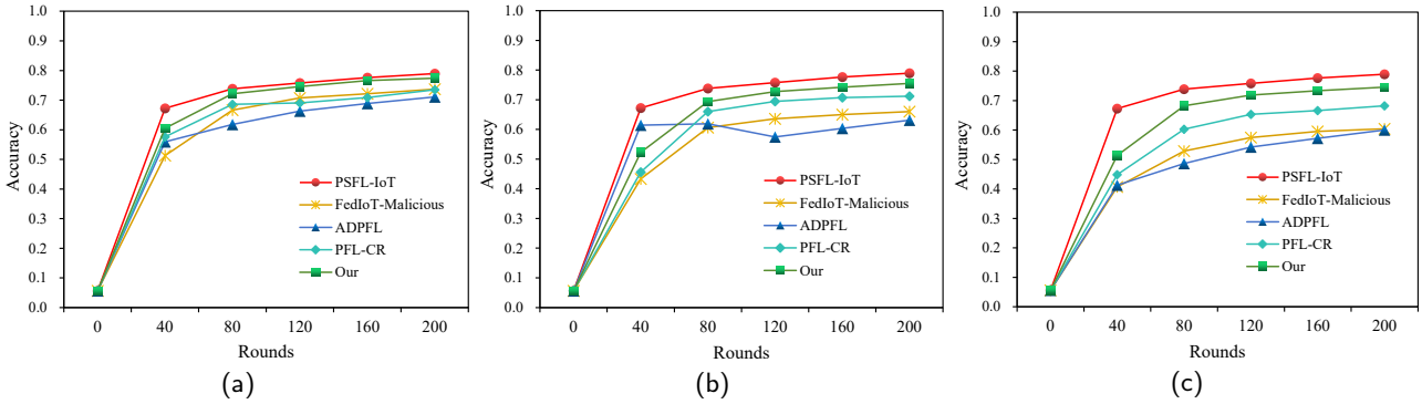
Figure 5: Comparison of Model Performance Under Data Pollution Attacks on FMNIST Dataset.
